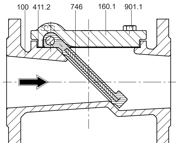
Horizontal installation position 6) (Shown: variant without lining)
