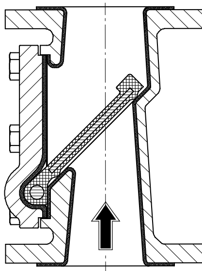
Vertical installation position 7) (Shown: variant with lining)
