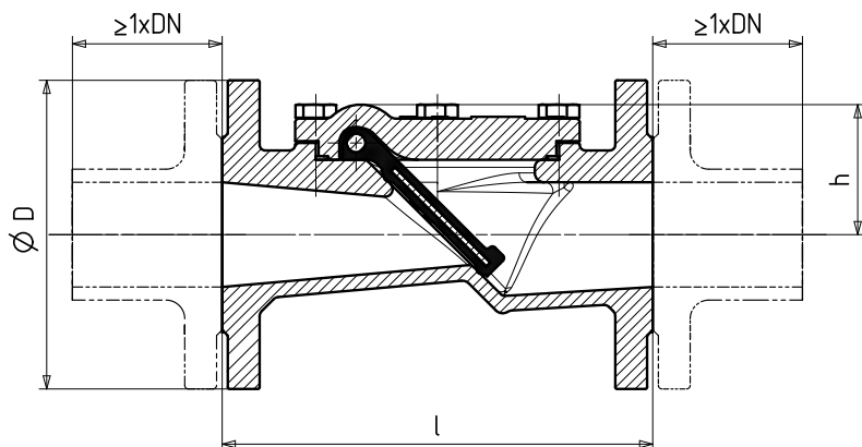
Front view / Sectional drawing with upstream/downstream stabilisation distance
