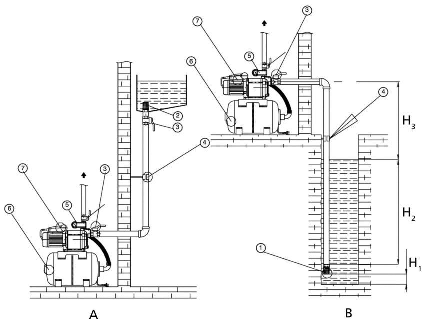
Fig. 2: Installation drawing
