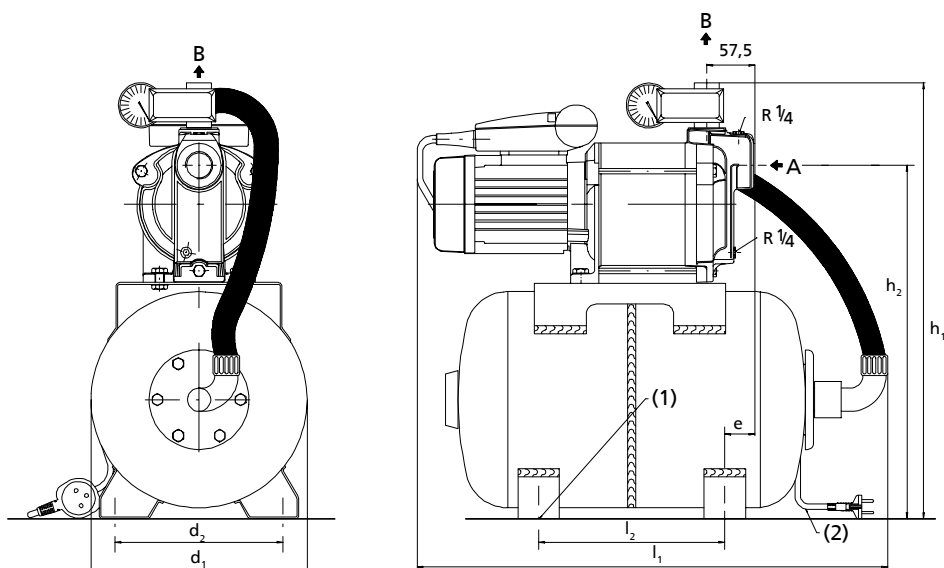
Fig. 1: Dimensions [mm]
