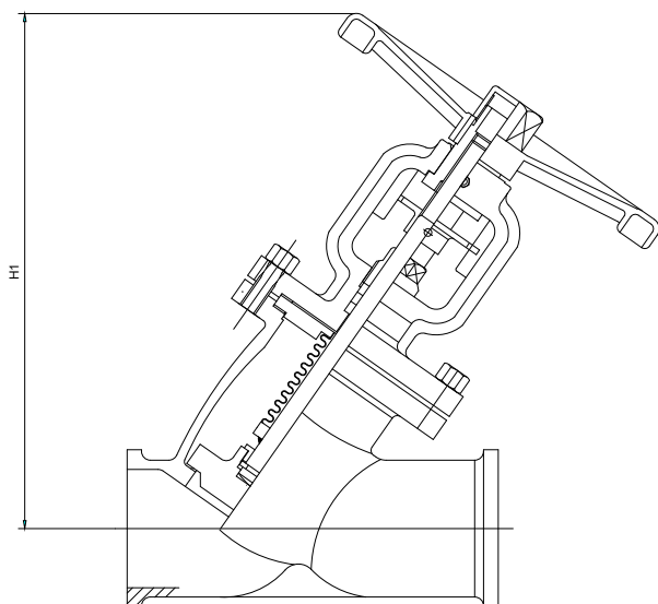
Fig. 3: Dimensions of BOACHEM-ZYAB
