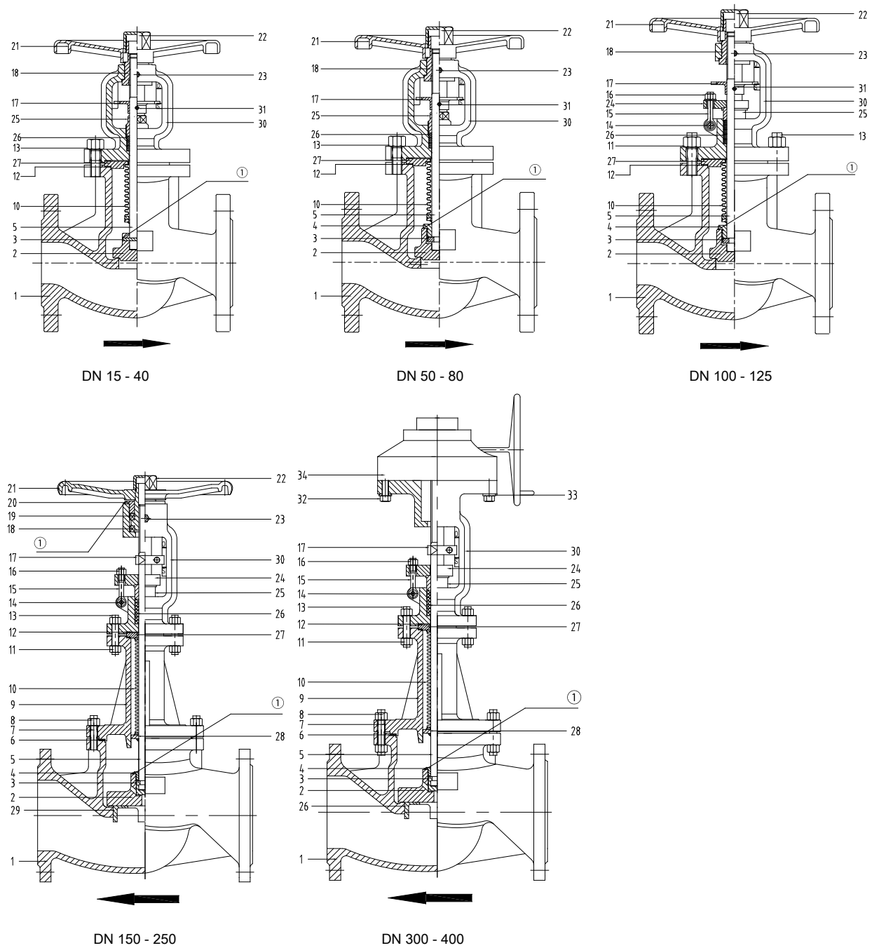
Fig. 1: Sectional drawings
