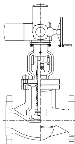
Mounting of electric actuator
