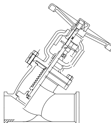
Straight-way Y-valve
