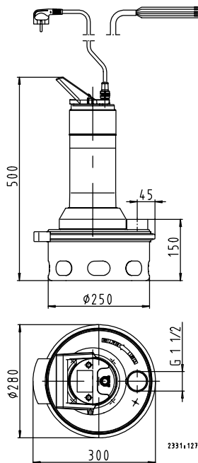
Fig. 2: AmaDrainer 4, free passage 35 mm, without cooling jacket
