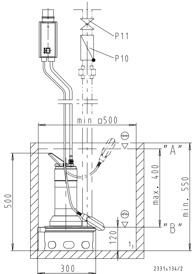
Fig. 6: AmaDrainer 4, single pump, free passage 35 mm, with float switch, three-phase motor, without cooling jacket
