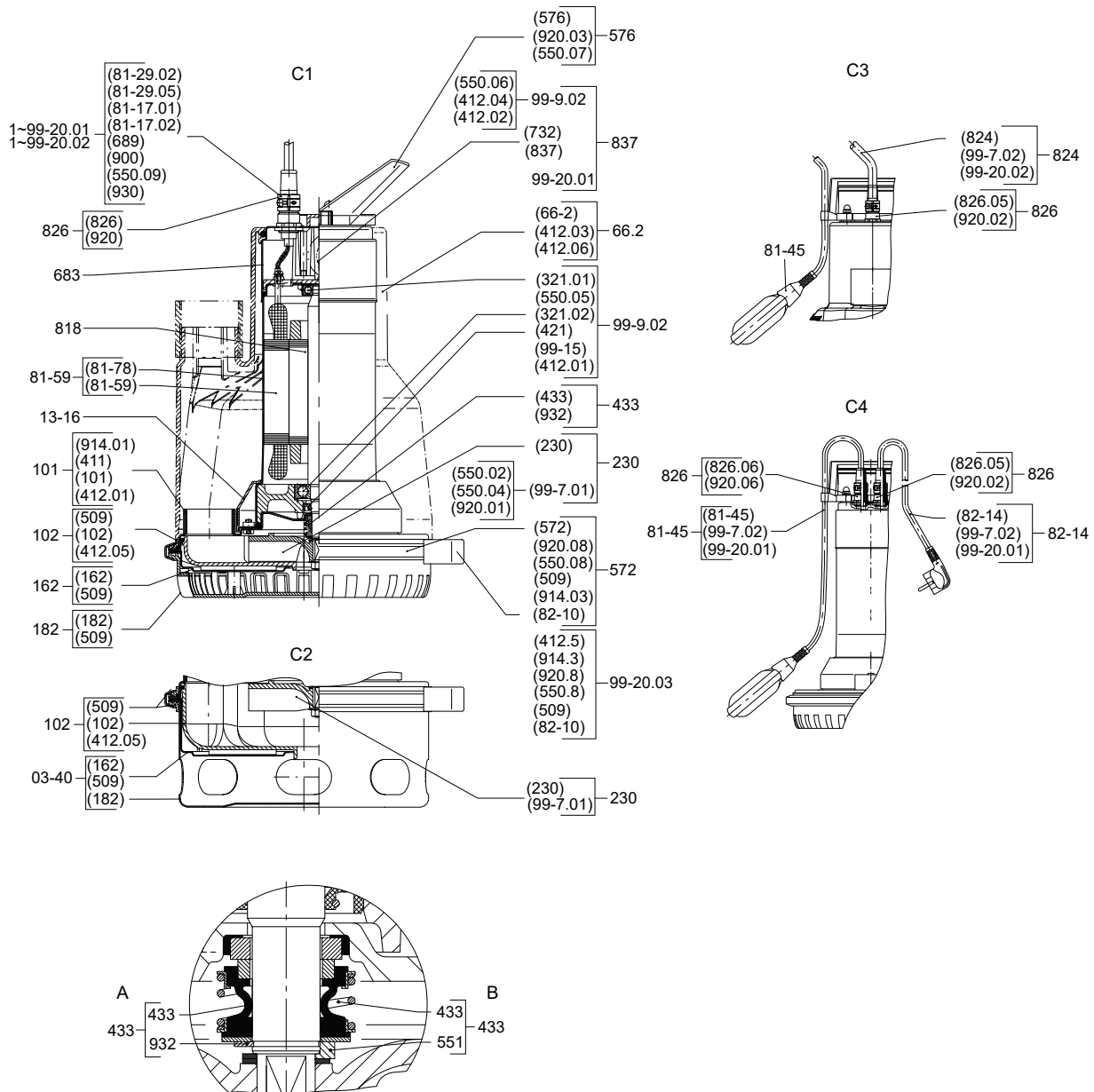
Fig. 15: General assembly drawing of AmaDrainer .../10, .../10K, .../35
