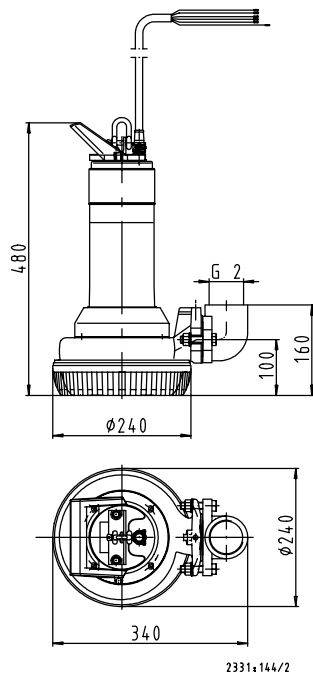
Fig. 4: AmaDrainer 5, free passage 11 mm, without cooling jacket
