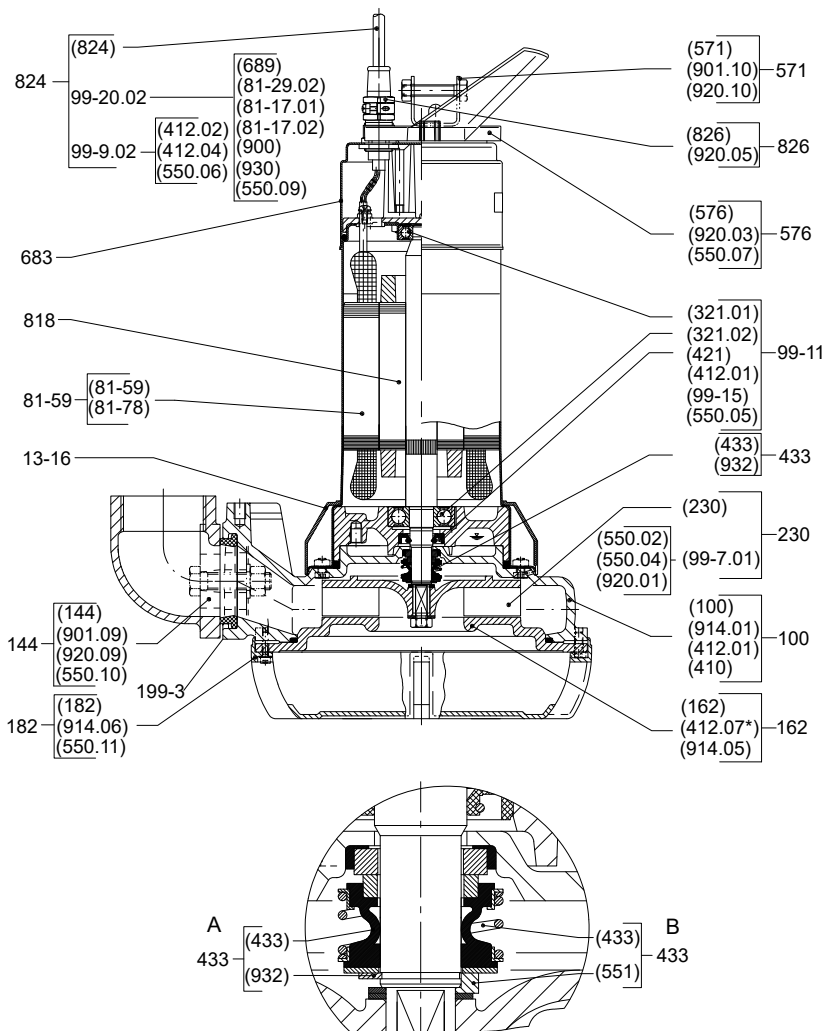
Fig. 16: General assembly drawing of AmaDrainer 522/11
